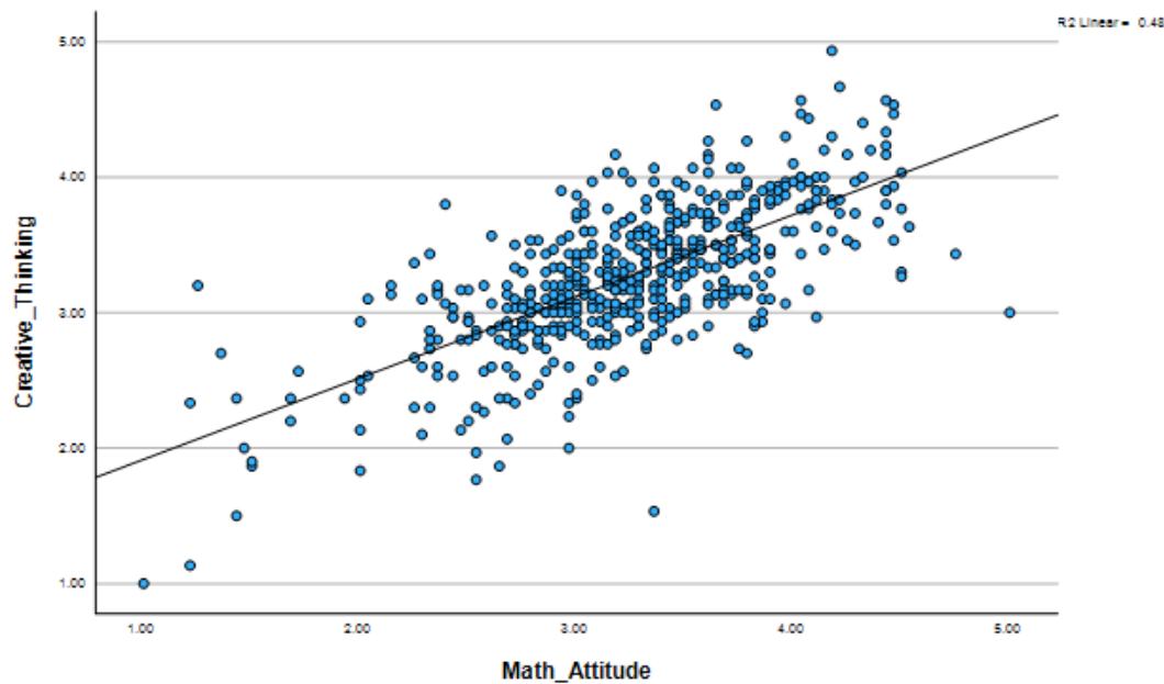
Figure 2: Scatter plot of mathematics attitude and creative thinking
