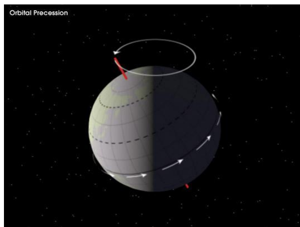
Fig. 5 Wobbling of the Earth's axis in the anti-clockwise direction. Its spin direction is also shown to be anticlockwise ( http://earthobservatory.nasa.gov/IOTD/view.php?id=541 )
