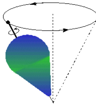
Fig. 4. Precession of spinning top that traces the surface of a cone. It spins and wobbles in the anticlockwise direction ( http://www-istp.gsfc.nasa.gov/stargaze/Sprecess.htm )
