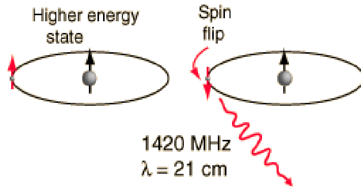
Fig. 24. Electron spin flip ( http://hyperphysics.phy-astr.gsu.edu/hbase/quantum/h21.html )
