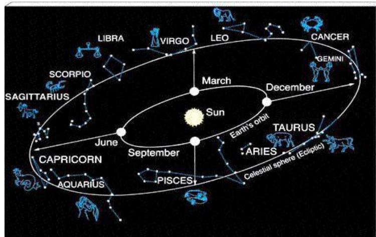
Fig. 17. Path through the constellations ( http://www.astro.psu.edu/users/caryl/a10/lec2_2d.html )
