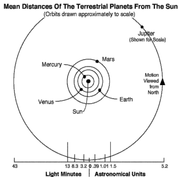
Fig. 11. Asteroids go round the sun in the anticlockwise direction. ( www.solarviews.com )
