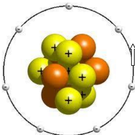
Fig.. 20. In a binary star system, both stars move around their center-of-mass indicated by a + sign. . ( http://www.astro.cornell.edu/academics/courses/astro201/bin_orbits.htm )
