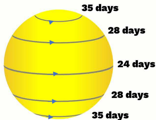
Fig.13. Spinning of the Sun ( https://astronomyrookie.com/is-the-sun-spinning/ )
