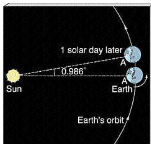
Fig. 3. Planet Earth's motion around the Sun in the anticlockwise direction. Its spin direction is also shown in the anticlockwise direction.
